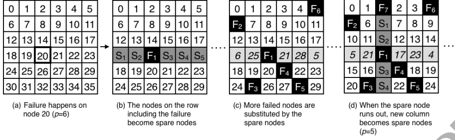
Figure 1: Example of node failures substituted by spare nodes in a 2-D GRIDSHAPED application.
